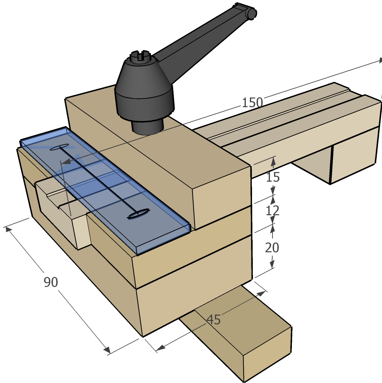
General View Narrow ripping setting jig www.workshopessentials.com
